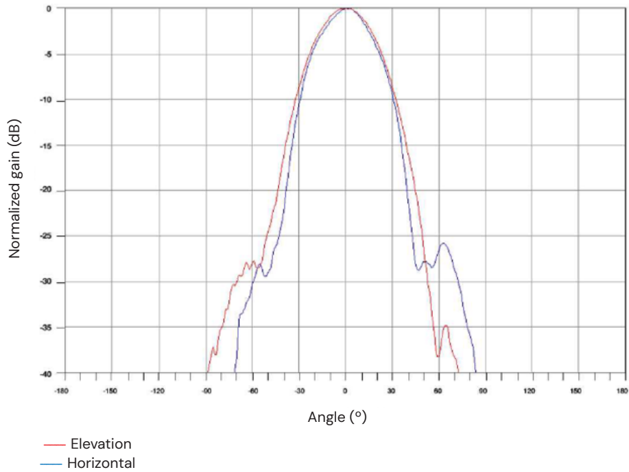
TX – Antenna Pattern
