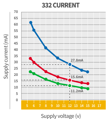
FIG 1: SUPPLY CURRENT VS. SUPPLY VOLTAGE
